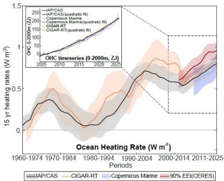
Fig. 2. Running 15-year ocean heating rates and uncertainties for the IAP/CAS, CIGAR-RT, Copernicus Marine, and CERES satellite observations of the net TOA radiation (units: \text{Wm}^{-2} ). For the observational datasets and reanalysis data, uncertainties are represented by twice the standard deviation of ensemble warming rates for each product. All heating rates are expressed per unit area of Earth’s surface ( 5.1 \times 10^{14} \text{ m}^2 ). The inset displays the annual OHC time series (colored solid lines) and the quadratic fits to the OHC (colored solid lines with circle markers) over 2005–2025, relative to the 2005–2009 baseline (units: ZJ).
